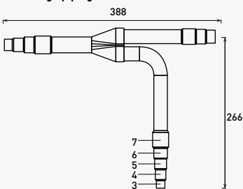
Discharge piping
