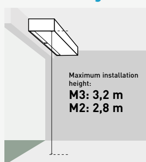
Suspended (standard)
