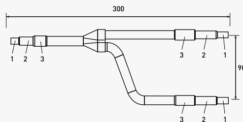
Liquid piping
