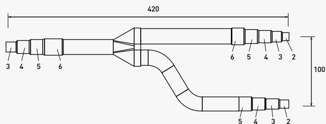
Gas piping
