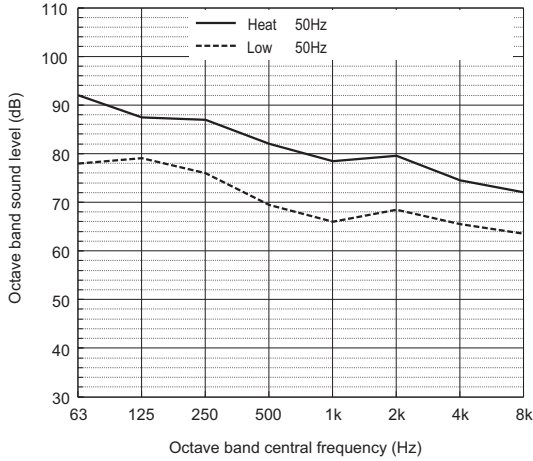
Sound power level of PUHY-M650YSXM-A
