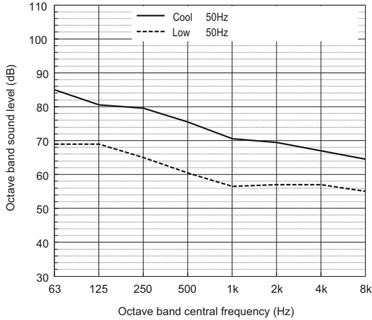
Sound power level of PUHY-M250YXM-A
