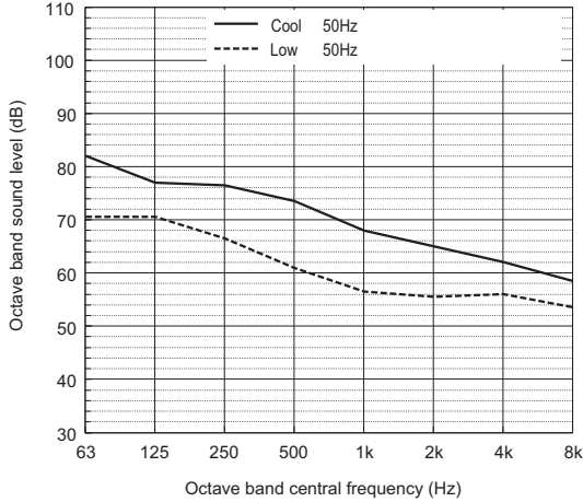
Sound power level of PUHY-M200YXM-A
