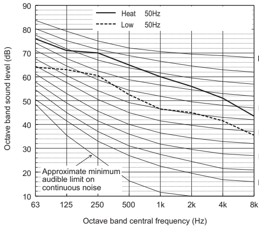
Sound level of PUHY-M650YSXM-A
