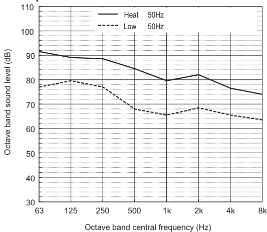
Sound power level of PUHY-M750YSXM-A
