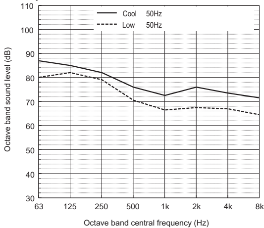
Sound power level of PUHY-M700YSXM-A
