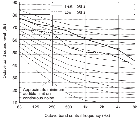
Sound level of PUHY-M800YSXM-A
