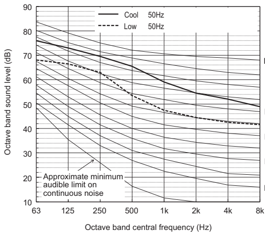
Sound level of PUHY-M900YSXM-A
