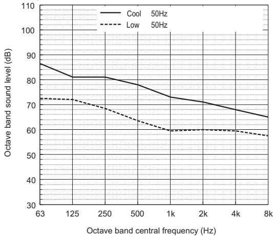
Sound power level of PUHY-M300YXM-A
