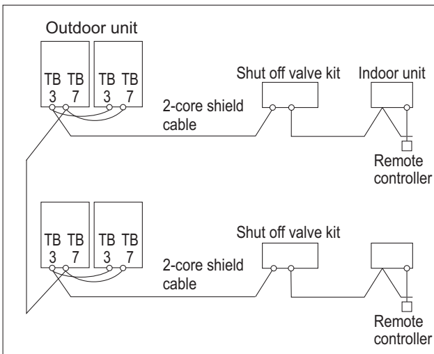
TB3:Terminal block for Indoor/Outdoor transmission cable TB7:Terminal block for central control transmission cable
