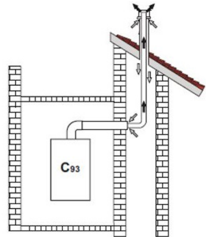
example of connection to collective flues
