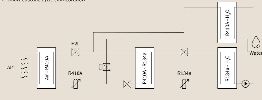
Fig. 1: Smart Cascade cycle configuration
