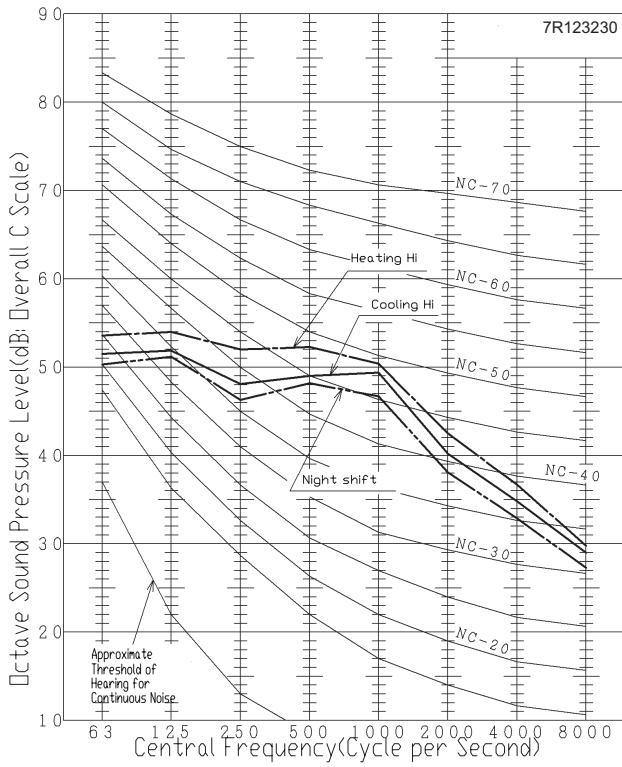
Cooling/Heating/Night mode: 52/54/50 dB(A)
