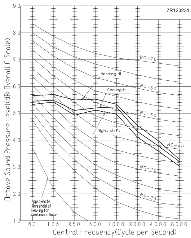
Cooling/Heating/Night mode: 55/57/53 dB(A)
