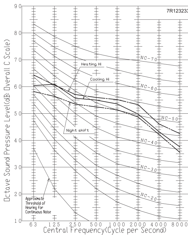
Cooling/Heating/Night mode: 58/60/56 dB(A)
