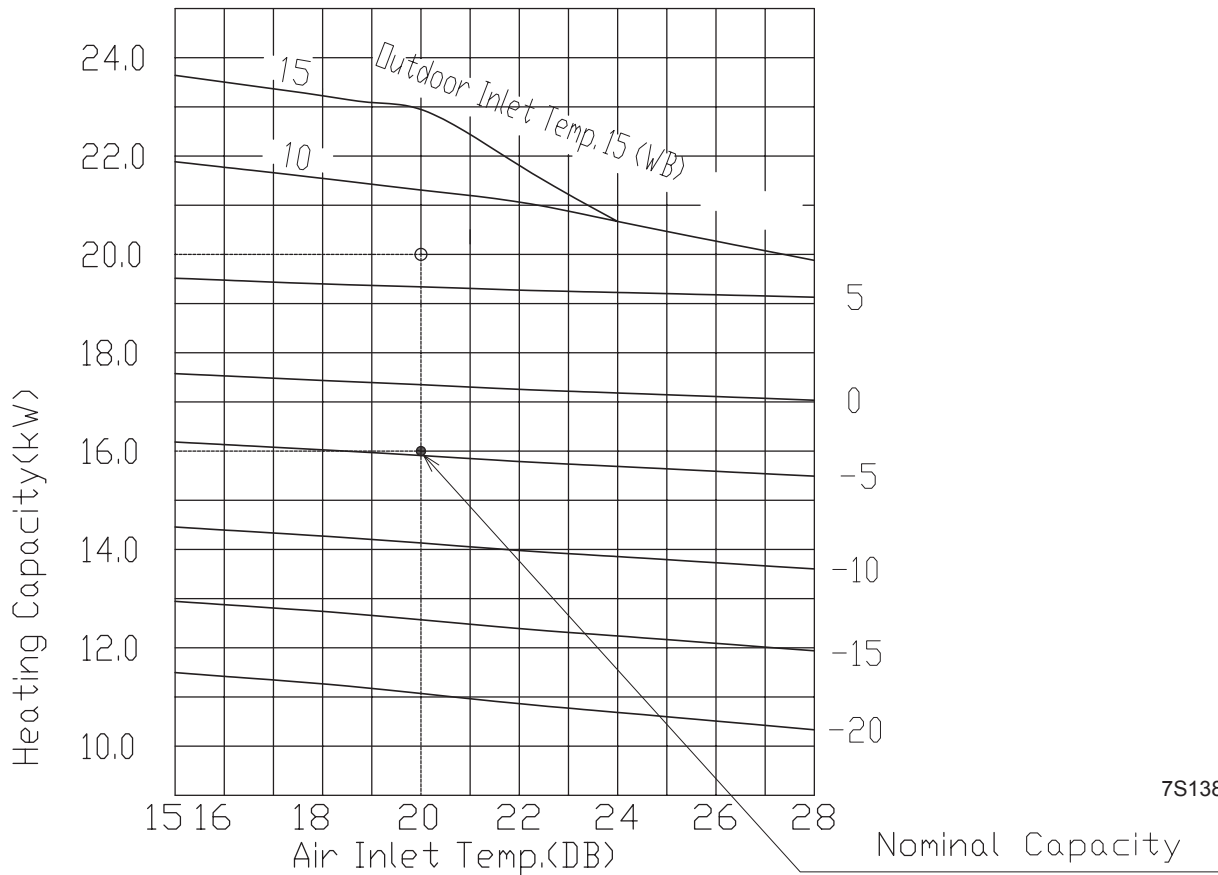
Heating Capacity curves
