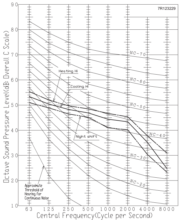
Cooling/Heating/Night mode: 50/52/48 dB(A)
