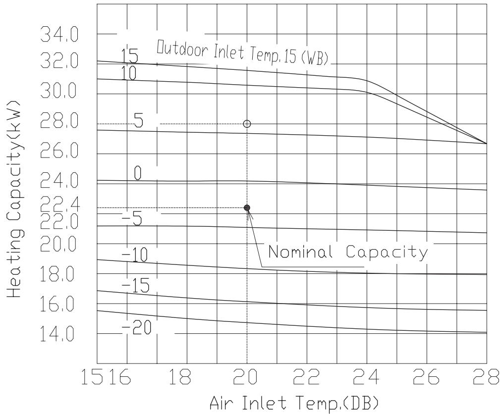
Heating Capacity curves
