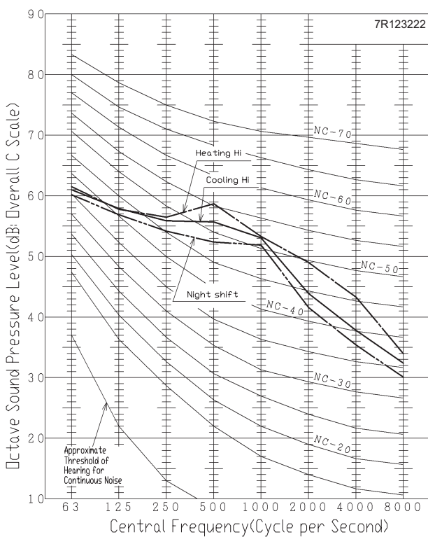
Cooling/Heating/Night mode: 57/59/55 dB(A)
