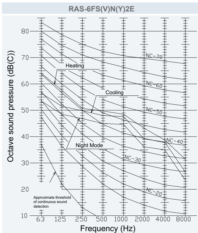
Sound pressure level: Cooling/Heating/Night mode; 51/53/48 dB(A)
