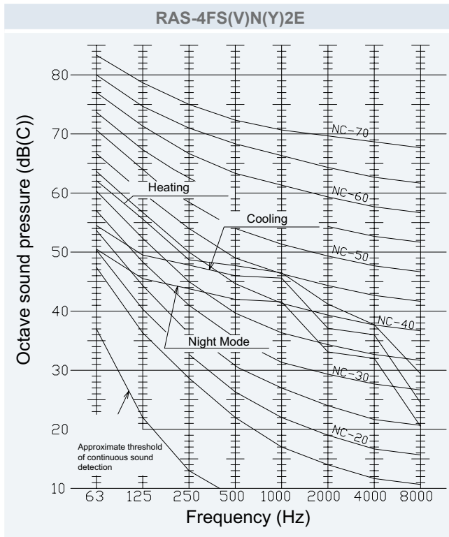
Sound pressure level: Cooling/Heating/Night mode; 49/51/45 dB(A)
