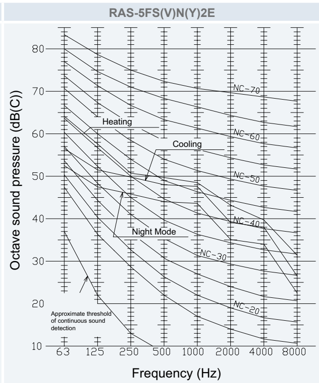
Sound pressure level: Cooling/Heating/Night mode; 51/53/47 dB(A)
